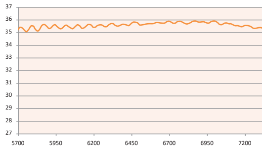
Antenna Gain 5700-7200 MHz
