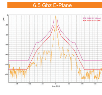
Antenna Gain 5700-7200 MHz
