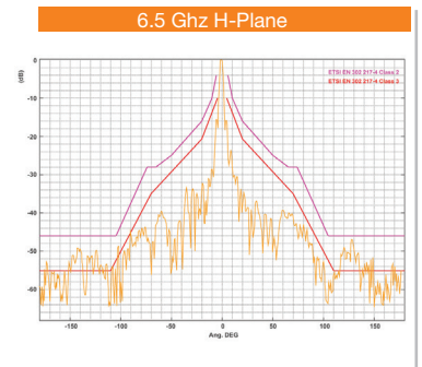
Antenna Gain 5700-7200 MHz
