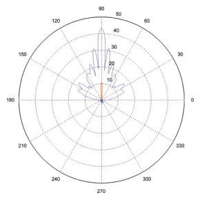
6.0 Ghz E-Plane and H of E-plane
