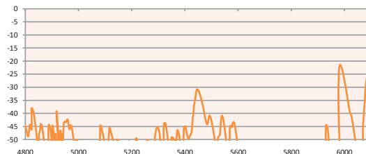
Antenna Port to Port Isolation 5400-6700 MHz
