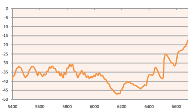
Antenna Cross Polarity 5400-6700 MHz
