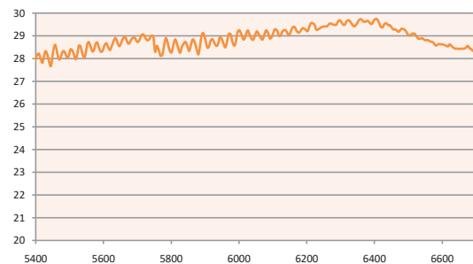
Antenna Gain 5400-6700 MHz
