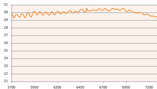
Antenna Gain 5700-7200 MHz
