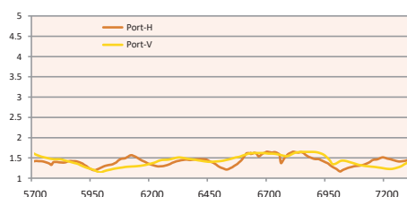
Antenna VSWR 5700-7200 MHz
