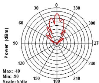
5.5 Ghz E-Plane and H of E-plane
